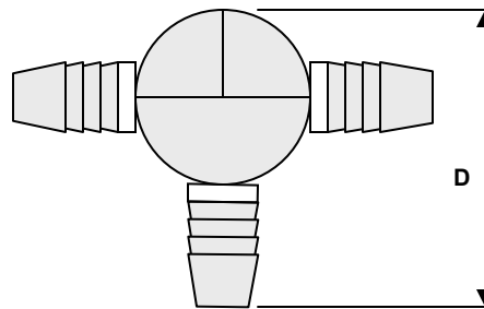
Top plan view without lever
